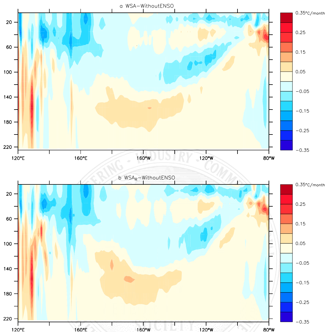
FIG. 7. Time-mean NDH difference as function of depth and longitude along equator (a) between the runs with ENSO (WSA) and without ENSO and (b) between the runs with reversed ENSO (WSA_R) and without ENSO. Presented are the annual means ( ^{\circ}\text{C month}^{-1} ).
