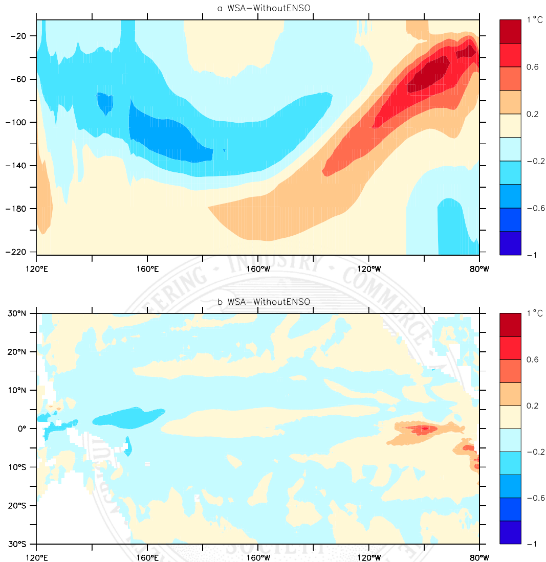
FIG. 3. Differences in the time-mean equatorial (a) upper-ocean temperature (5°N–5°S) and SST (b) between the runs with ENSO (WSA) and without ENSO (control).
