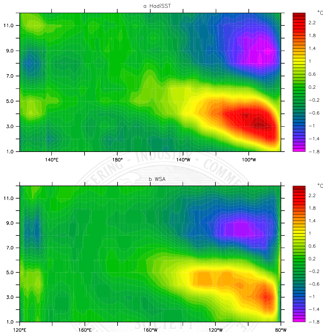
FIG. 2. The seasonal cycle in equatorial SST (5°N–5°S) from (a) observations (Rayner et al. 2003) and (b) WSA. Presented are the deviations from their respective annual mean SSTs.
