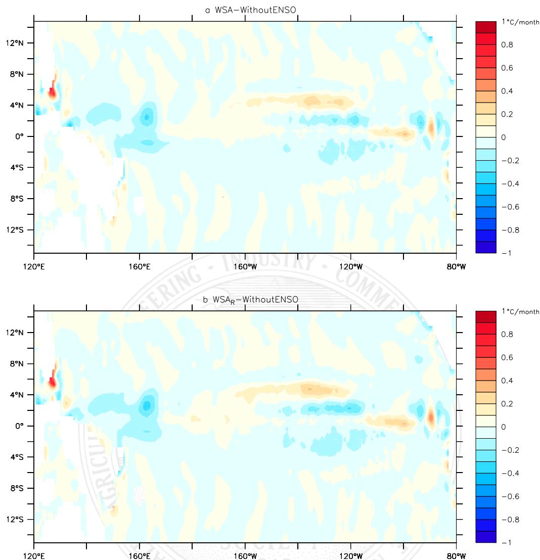
FIG. 8. Time-mean NDH difference for the surface layer as function of latitude and longitude (a) between the runs with ENSO (WSA) and without ENSO and (b) between the runs with reversed ENSO (WSA_R) and without ENSO. Presented are the annual-mean values ( ^{\circ}\text{C month}^{-1} ).
