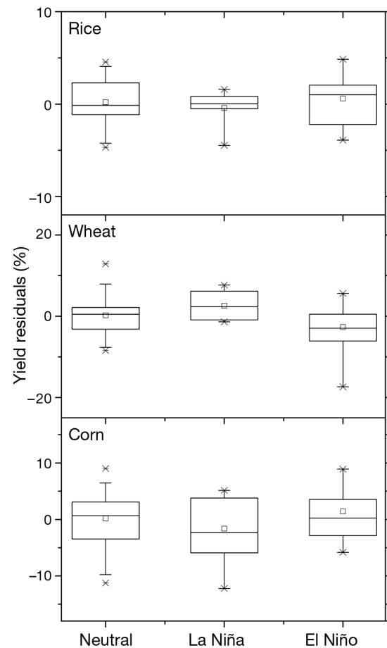
Fig. 8. Box plots showing 0, 25, 50, 75 and 100th percentiles and means (square) of national yield residuals with respect to ENSO phases in China, 1963–2008
