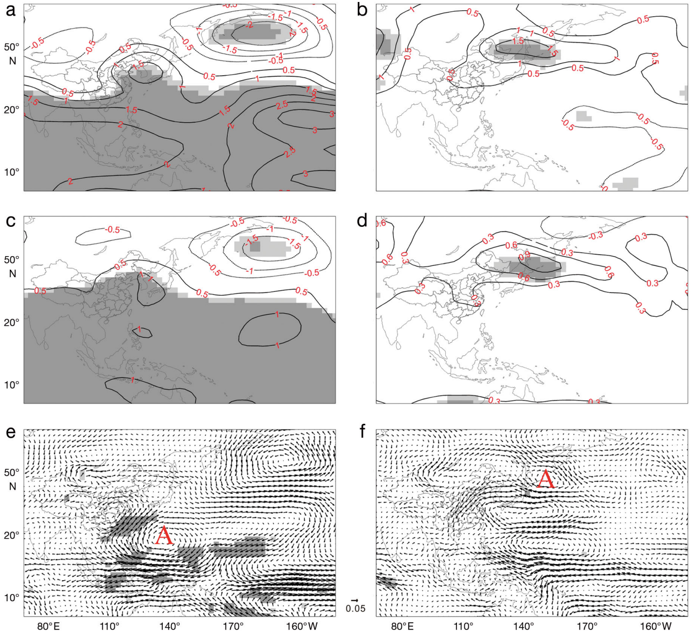
Fig. 7. Regression coefficient pattern of seasonal mean 200 mb geopotential height in (a) MAM(1) and (b) JJA(1), 500 mb geopotential height in (c) MAM(1) and (d) JJA(1), and 850 mb winds in (e) MAM(1) and (f) JJA(1) with respect to the ENSO index [left column: JJAS(0) SSTA; right column: JFMA(0) SSTA] for the period of 1962–2008. Light and dark shading indicate regions significant at the 95 and 99% confidence levels, respectively. Symbol 'A' indicates an anomalous anticyclone. Contour lines are regression coefficients
