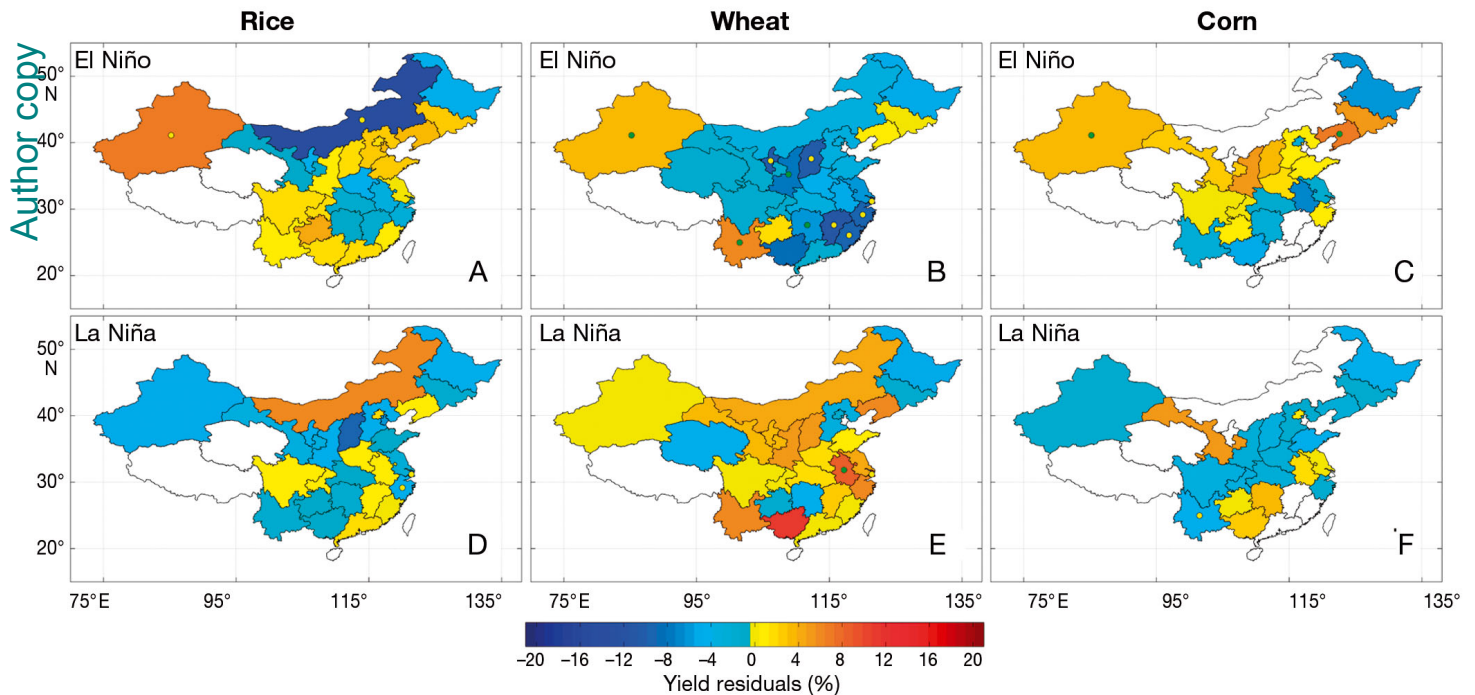
Fig. 4. Difference in yield residuals (%) for rice (A,D), wheat (B,E), and corn (C,F) in El Niño or La Niña years compared to neutral years). Provinces where the differences reach the 90 and 95% confidence levels are marked with green and yellow points, respectively
