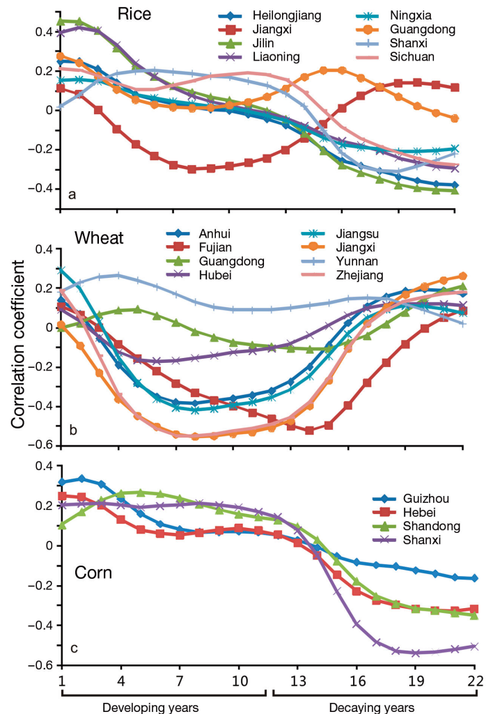
Fig. 6. Correlations between crop yield and the 3 mo sliding ENSO index from the beginning of the developing year to the end of the decaying year during 1962–2008
