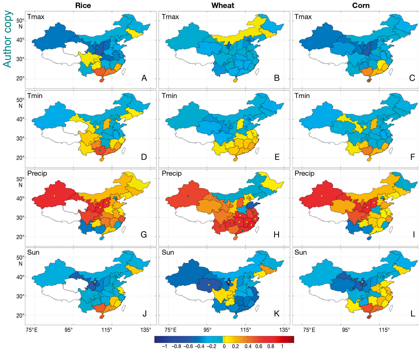
Fig. 2. Differences in climate variables during the growing season in El Niño years compared to neutral years: (A–C) maximum temperature, T_{\max} ; (D–F) minimum temperature, T_{\min} ; (G–I) precipitation; and (J–L) sunshine duration, S . Provinces where the differences in climate variables reached the 90 and 95% confidence levels are marked with green and yellow points, respectively. Color scale: difference after standardization of data to zero mean and unit variance
