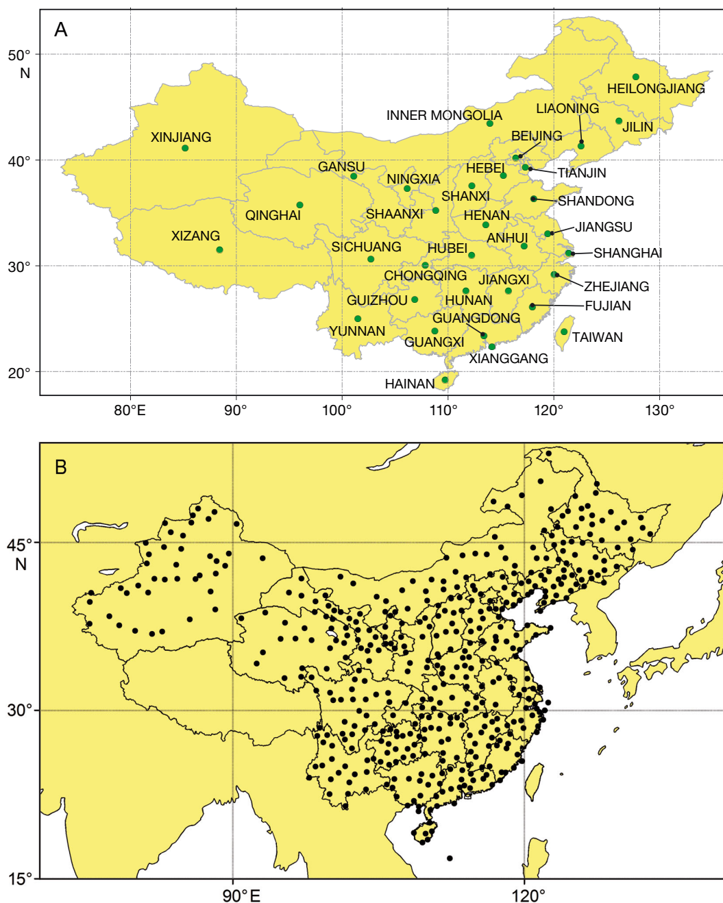
Fig. 1. (A) Provinces of China, covered in this study. (B) Distribution of weather stations used to calculate the province-averaged climate parameters. No stations in Xizang and Shanghai Provinces were used due to the lack of a continuous record
