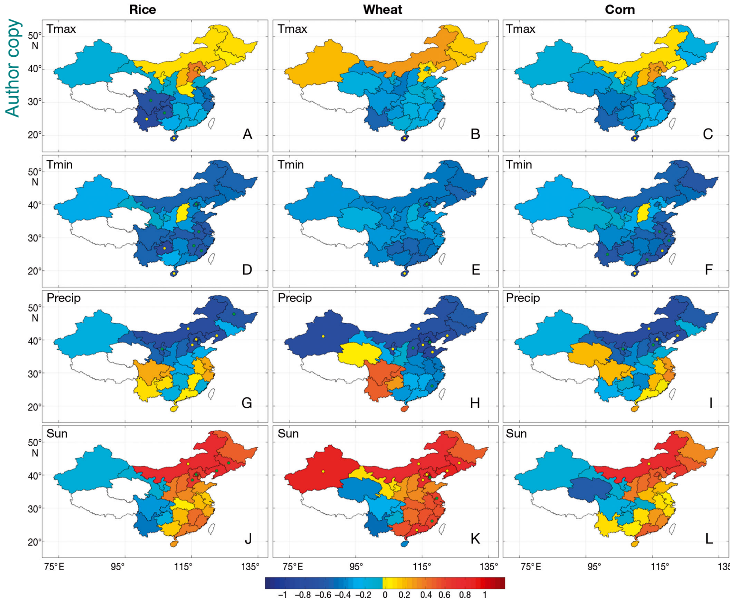
Fig. 3. Differences in climate variables during the growing season in La Niña years compared to neutral years: (A–C) maximum temperature, T_{max} ; (D–F) minimum temperature, T_{min} ; (G–I) precipitation; and (J–L) sunshine duration, S . Provinces where the differences reach the 90 and 95% confidence levels are marked with green and yellow points, respectively. Color scale: difference after standardization of data to zero mean and unit variance
