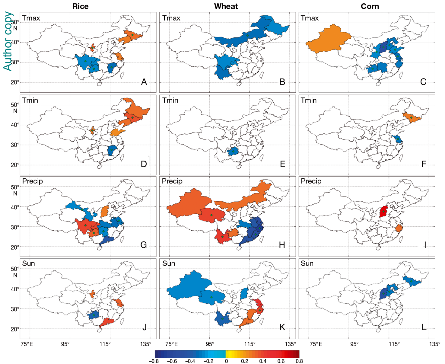
Fig. 5. Correlation between climate variables [(A–C) maximum temperature, T_{\max} ; (D–F) minimum temperature, T_{\min} ; (G–I) precipitation; and (J–L) sunshine duration, S ] during the growing season and yield residuals. Only statistically significant ( p < 0.10 ) correlations are shown. Provinces with a significant Granger causal relationship ( p < 0.10 ) are marked with a green point. Color scale: value of correlations
