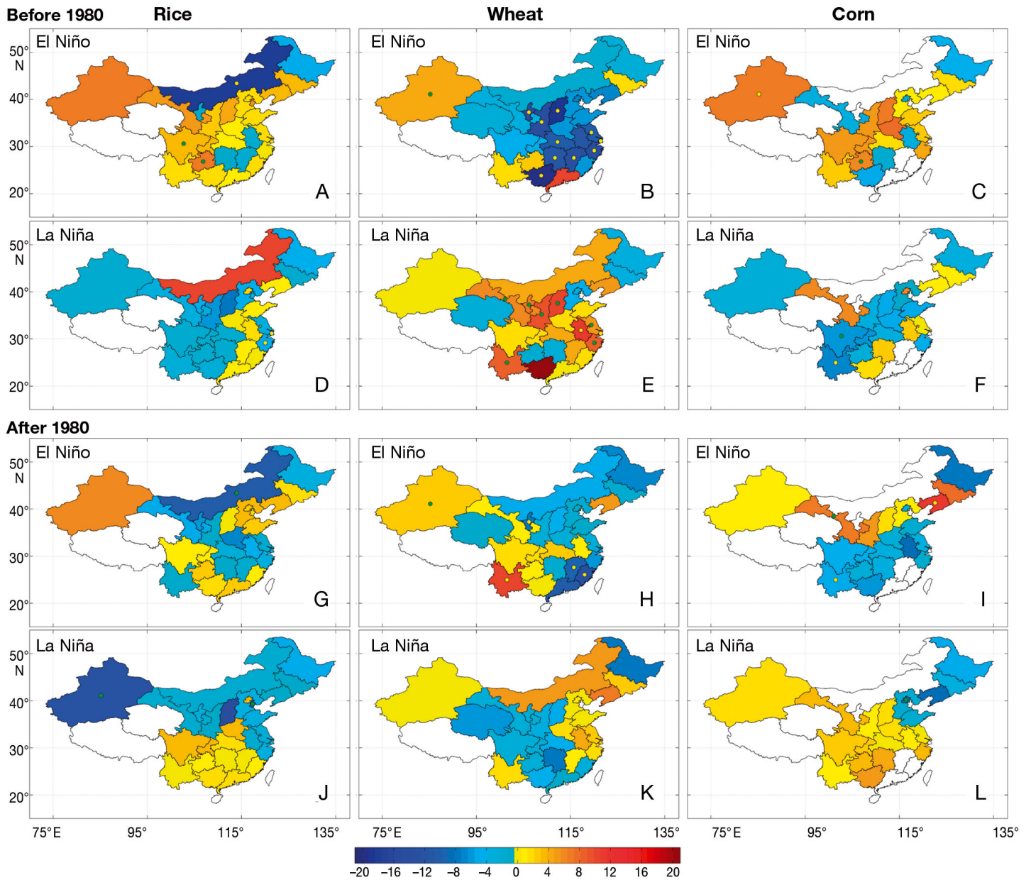
Fig. 9. Difference in yield residuals (%) in El Niño and La Niña years, compared to neutral years, for 1962–2008. Provinces where the differences reach the 90 and 95% confidence levels (ANOVA) are marked with green and yellow points, respectively. Color scale: difference in yield residuals (%)
