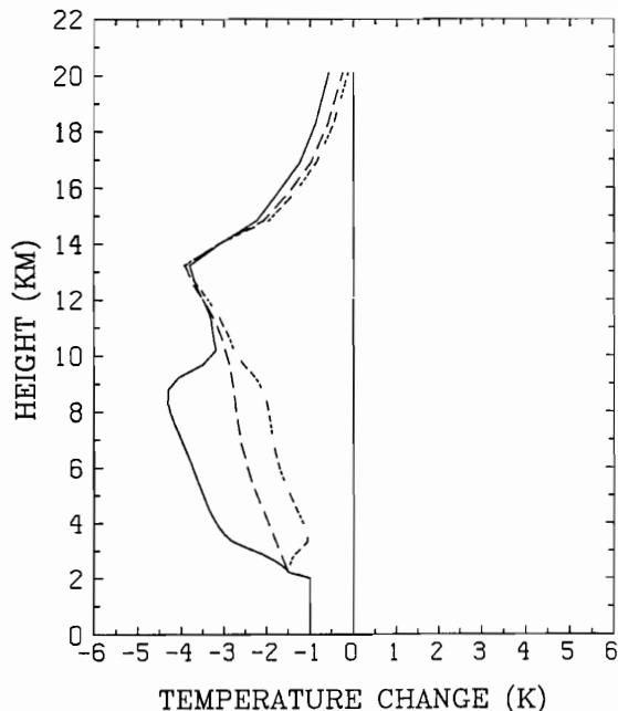
Fig. 4. Temperature change as a function of height when the surface temperature is decreased by 1 K. Long-dashed line : Relative humidity is fixed and is assumed not to change when the surface temperature is decreased by 1 K. Solid line : Relative humidity between 300 mb and 700 mb is assumed to increase by 0.2 when the surface temperature is decreased by 1 K. Short-dashed line : Relative humidity between 300 mb and 700 mb is assumed to be 80% of the present value
