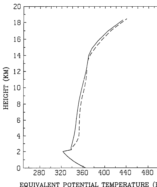
Fig. 3. Equilibrium saturation equivalent potential temperature, \theta^* . Solid line: fixed relative humidity; dashed line: fixed specific humidity
